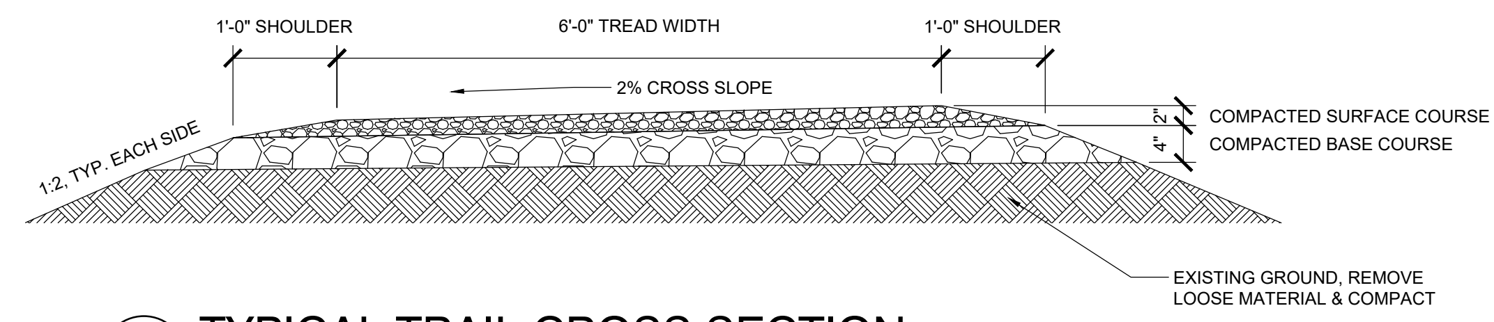
2 TYPICAL TRAIL CROSS SECTION A1.1 SCALE: 3/4" = 1'-0"
