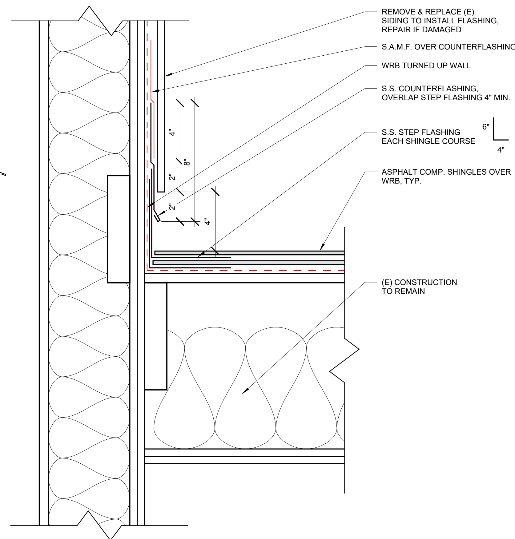
1 SIDEWALL FLASHING 3" = 1'-0"
