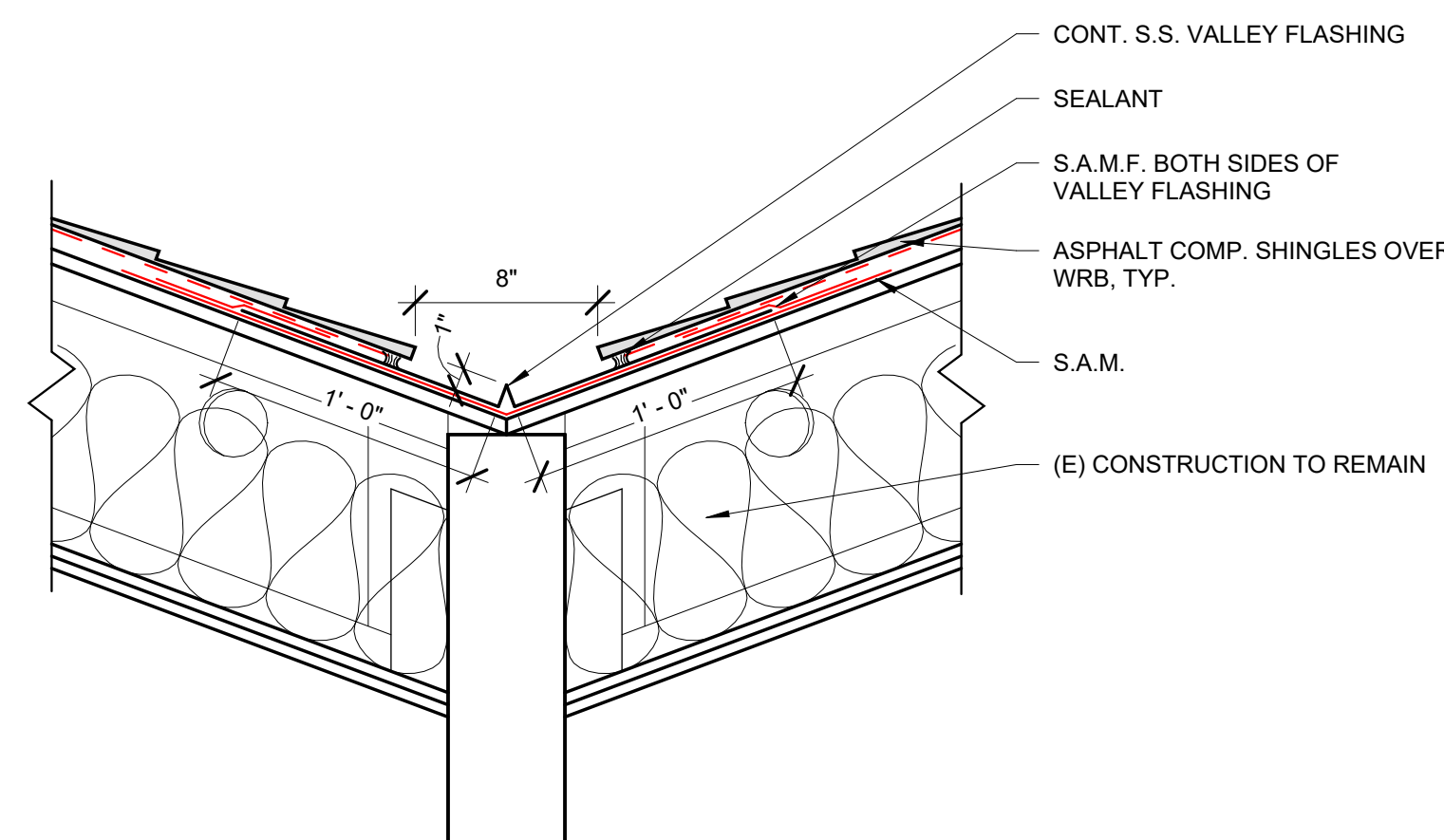
2 TYP. VALLEY FLASHING 1 1/2" = 1'-0"
