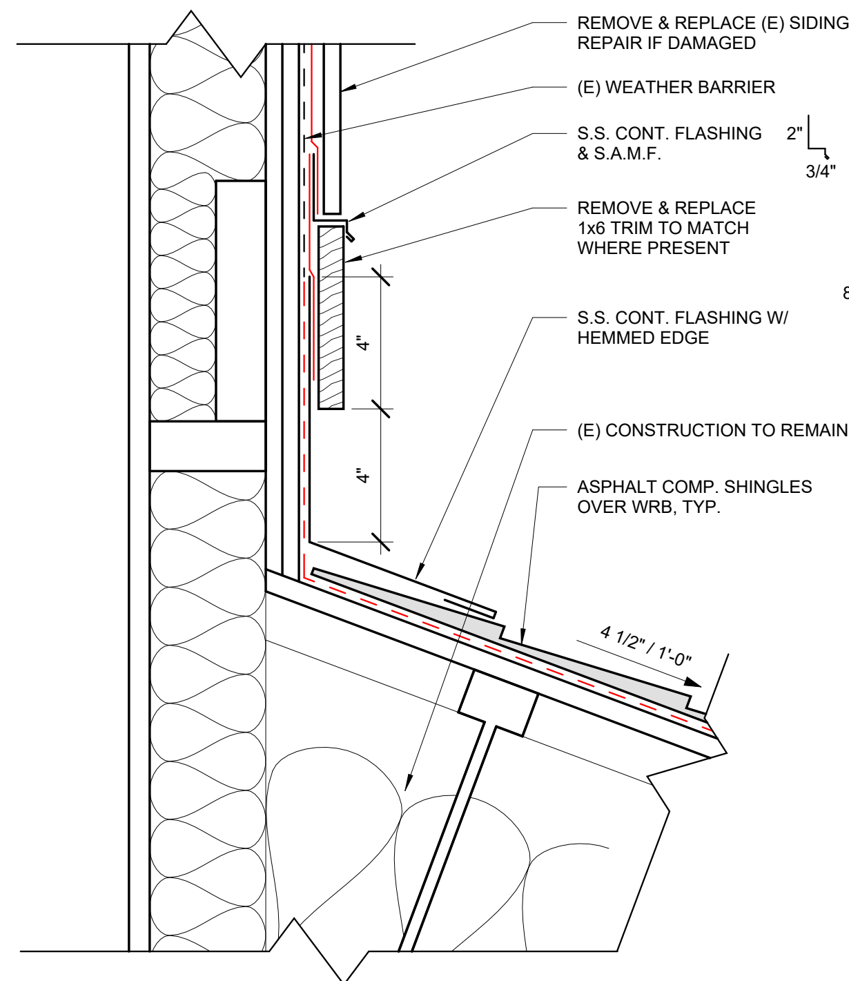
5 TYP. ROOF-WALL JUNCTURE 3" = 1'-0"
