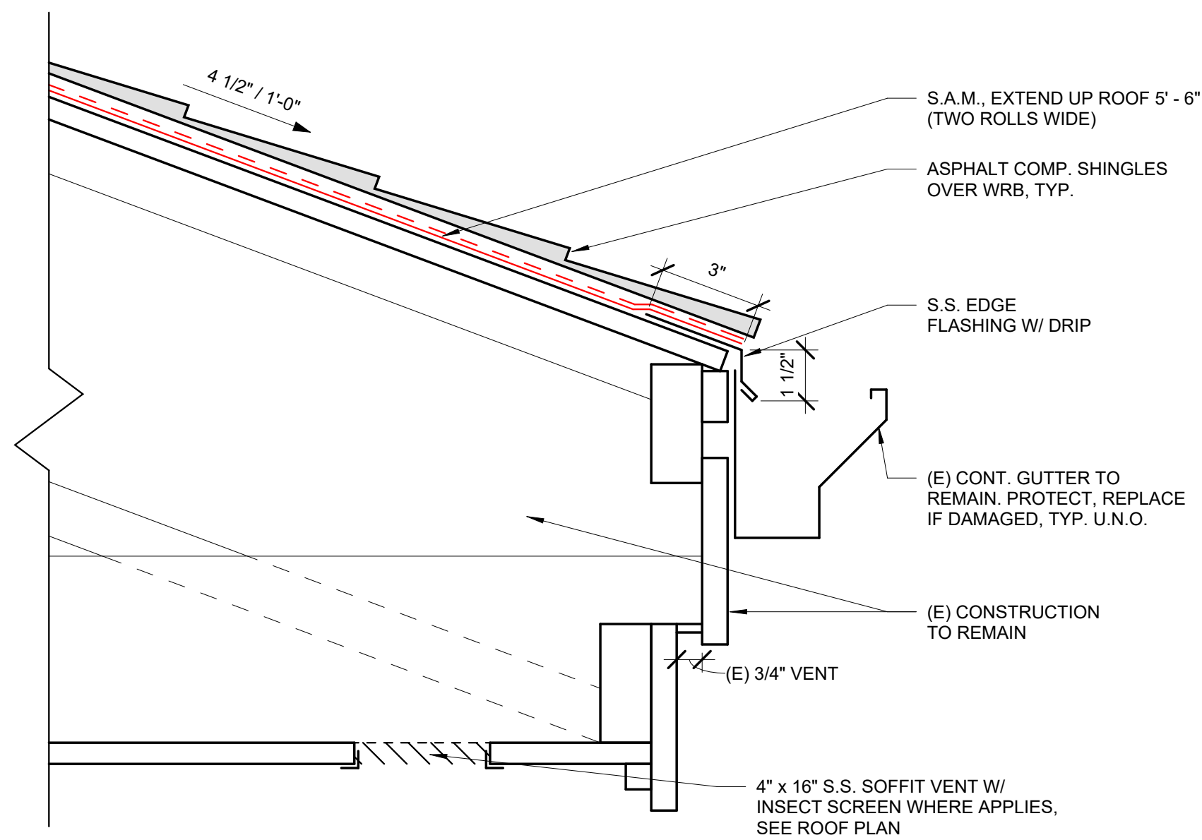
9 TYP. EAVE 3" = 1'-0"
