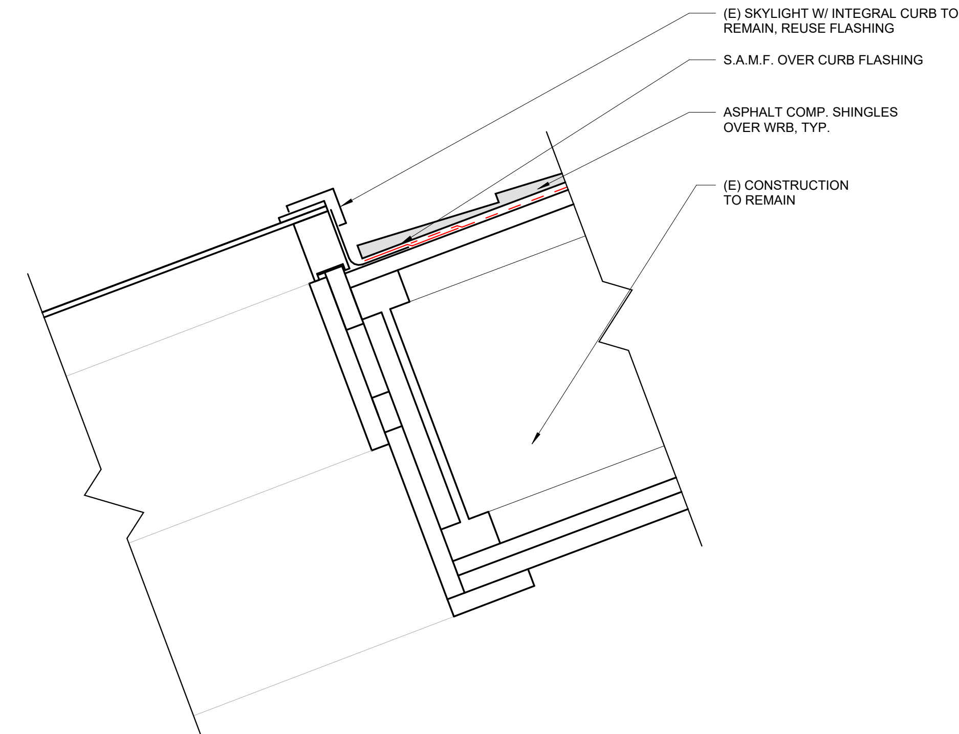
2 UPPER SKYLIGHT CURB 3" = 1'-0"
