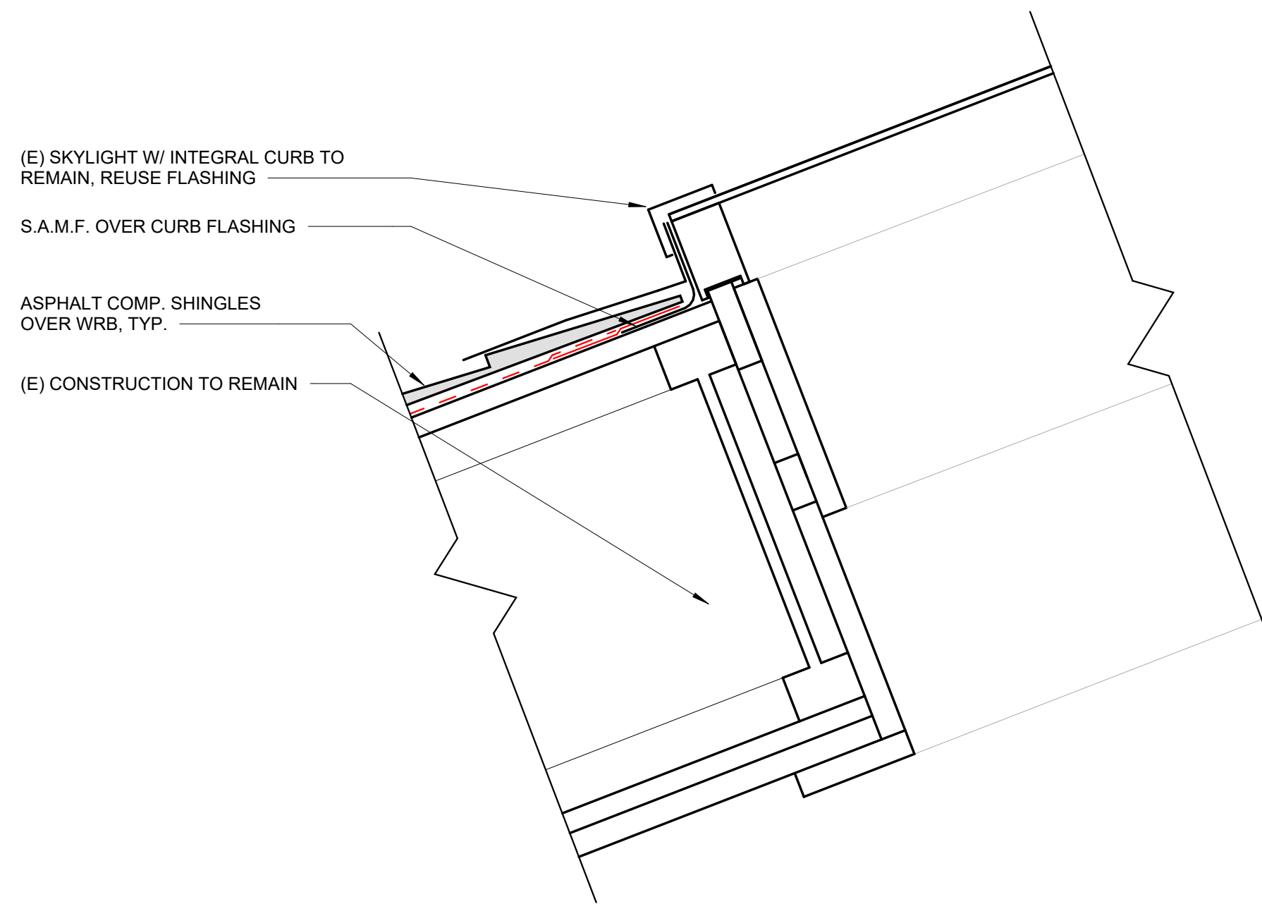
3 LOW SKYLIGHT CURB 3" = 1'-0"
