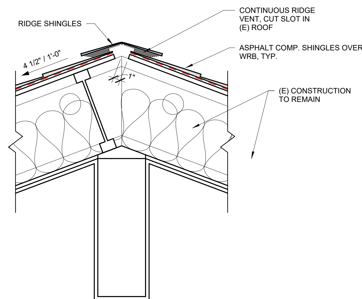
7 RIDGE VENT @ ATTIC 1 1/2" = 1'-0"
