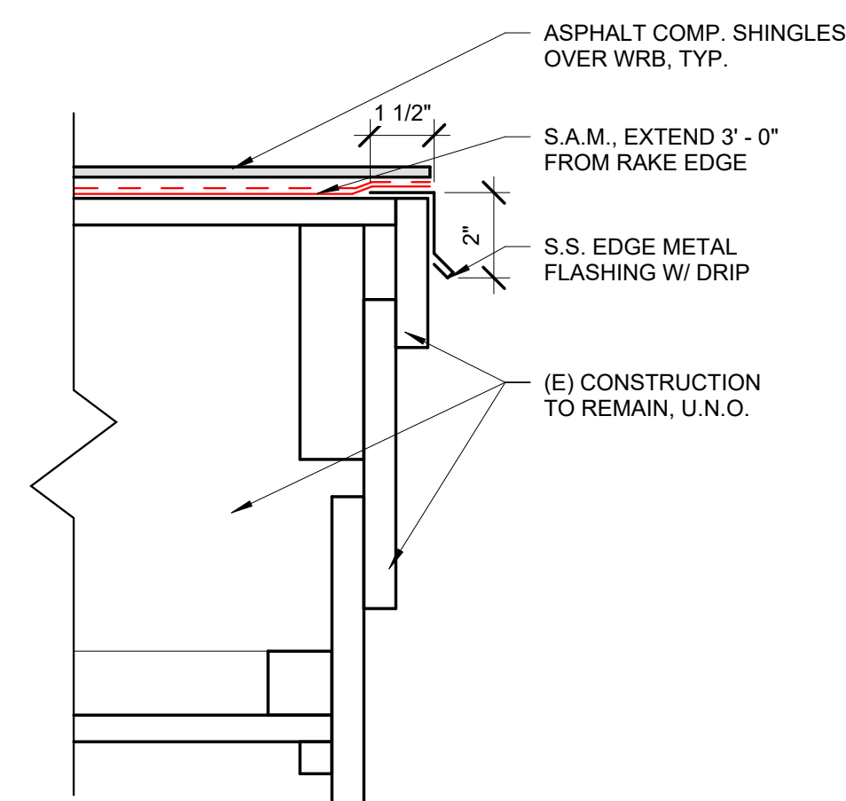
8 TYP. RAKE 3" = 1'-0"
