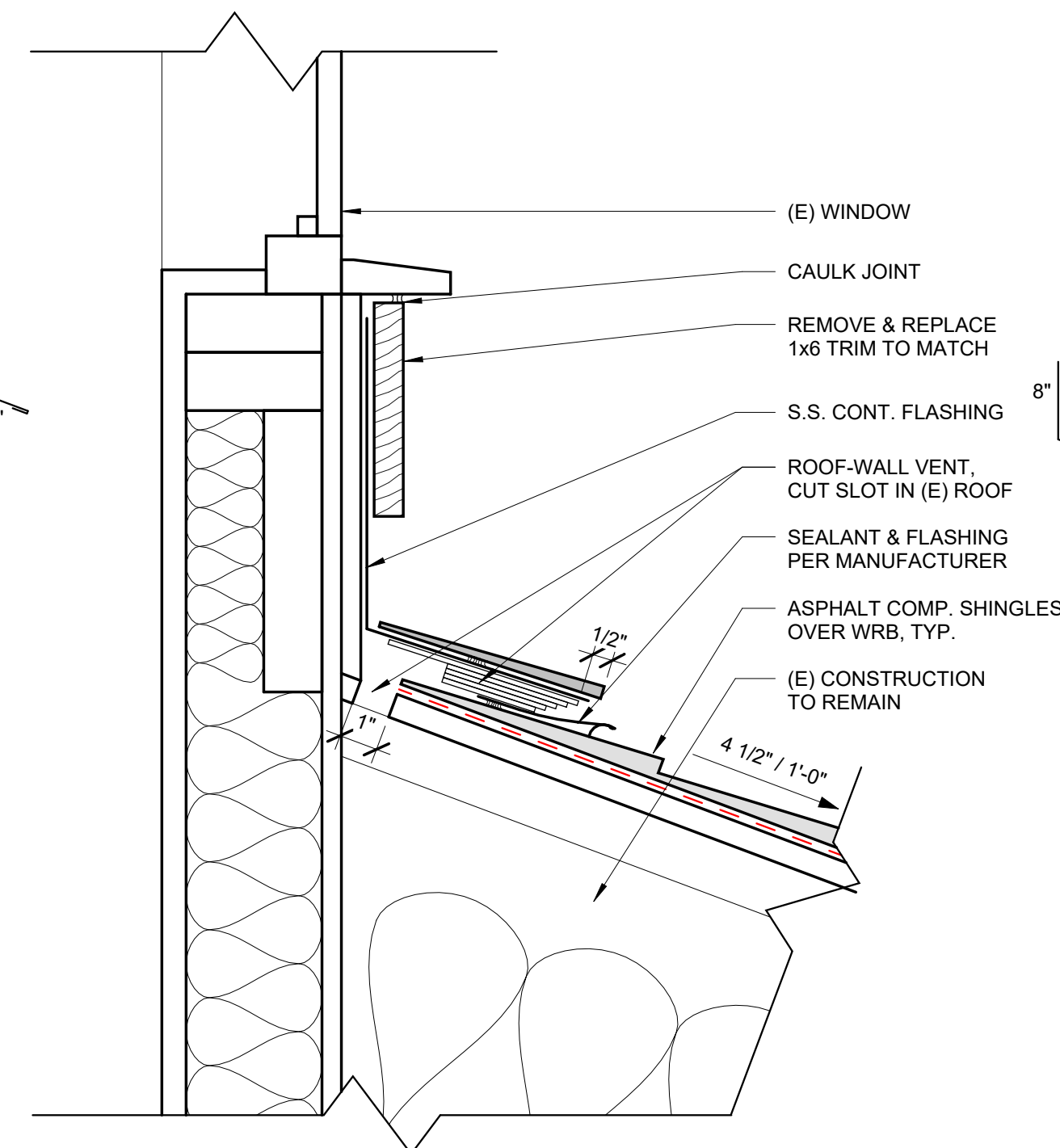
4 VENTED ROOF-WALL JUNCTURE 3" = 1'-0"
