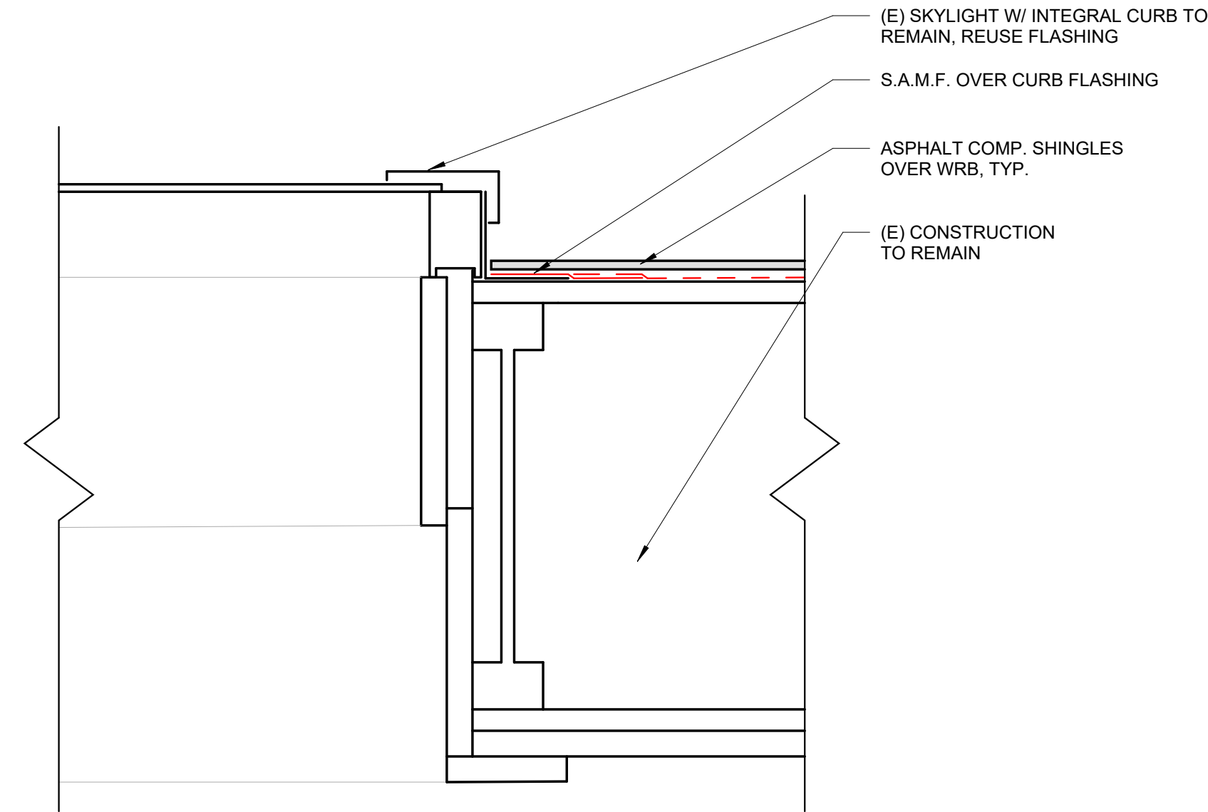
1 FLAT SKYLIGHT CURB 3" = 1'-0"
